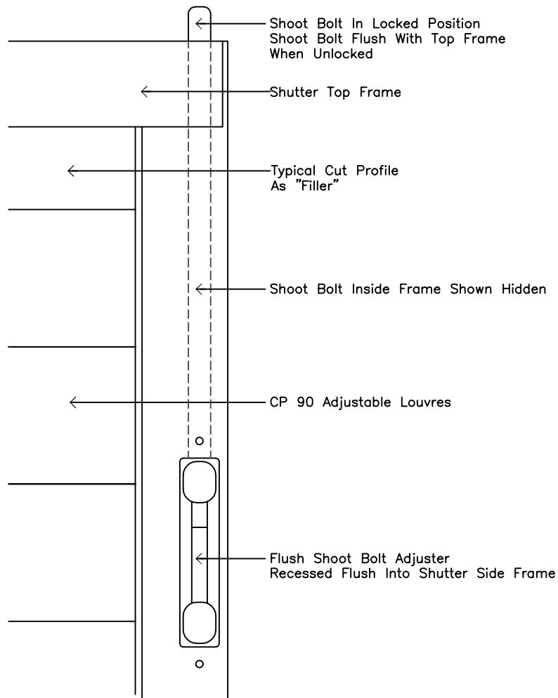
Flush Bolt Detail
