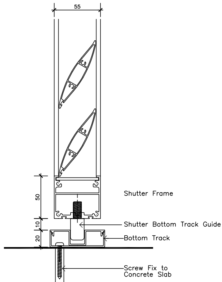
Fixed Blade Detail
