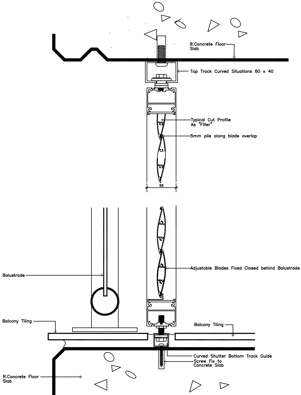
Bottom Track for Tiled Curved Balcony Detail
